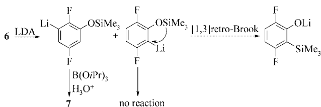
Scheme 3. LDA-induced rearrangement of 1,4-difluoro-2-(trimethylsilyloxy)benzene.
