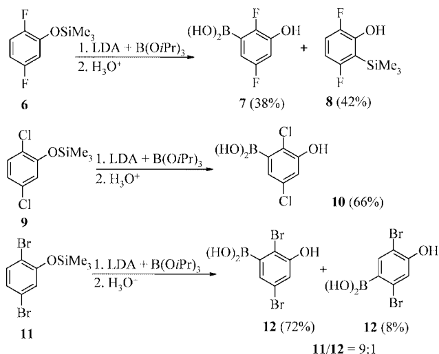
Scheme 2. Lithiation/boronation of 1,4-dihalo-2-(trimethylsilyloxy)benzenes.
