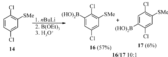
Scheme 4. Lithiation/boronation of 1,4-dichloro-2-(methylthio)benzene.
