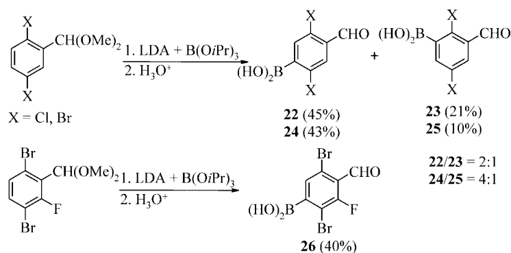
Scheme 6. Lithiation/boronation of 1,4-dihalo-2-(dimethoxymethyl)benzenes.
