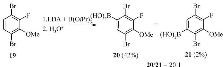
Scheme 5. Lithiation/boronation of 1,4-dibromo-2-fluoro-3-methoxybenzene.
