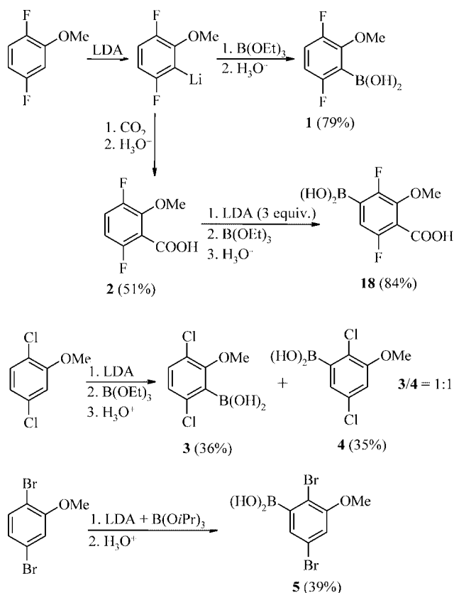
Scheme 1. Lithiation/boronation of 1,4-dihalo-2-methoxybenzenes.
